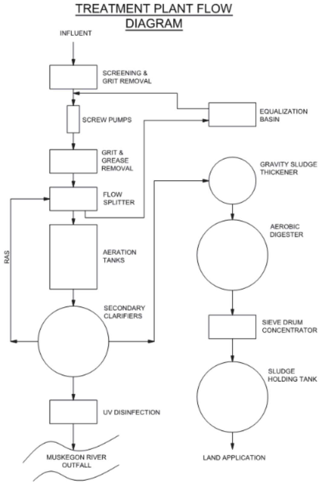
Figure 1: Big Rapids WWTP Flow Schematic
