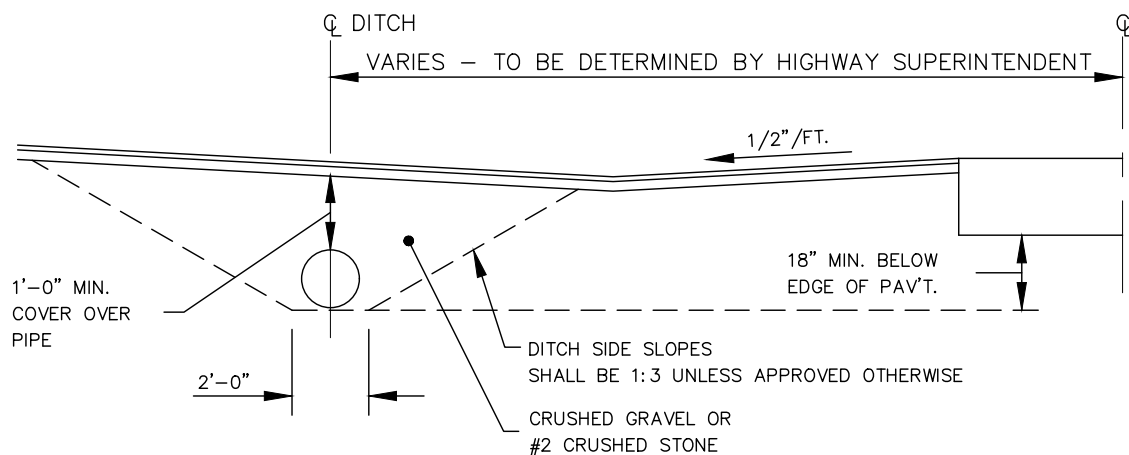
SECTIONAL VIEW
