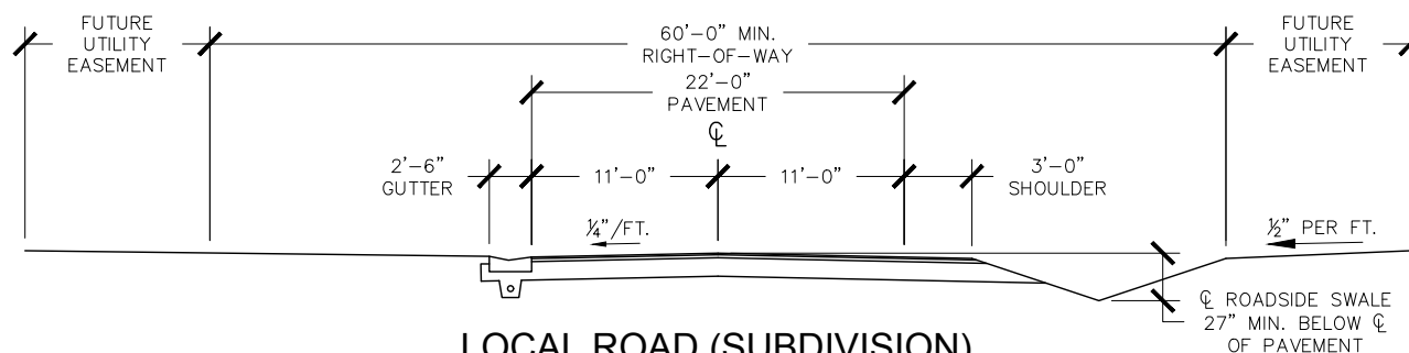
LOCAL ROAD (SUBDIVISION) (WITH CONCRETE GUTTER OR OPTIONAL SWALE)
