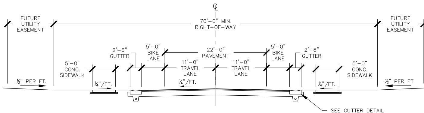
LOCAL ROAD (SUBDIVISION) (COMPLETE STREET)
