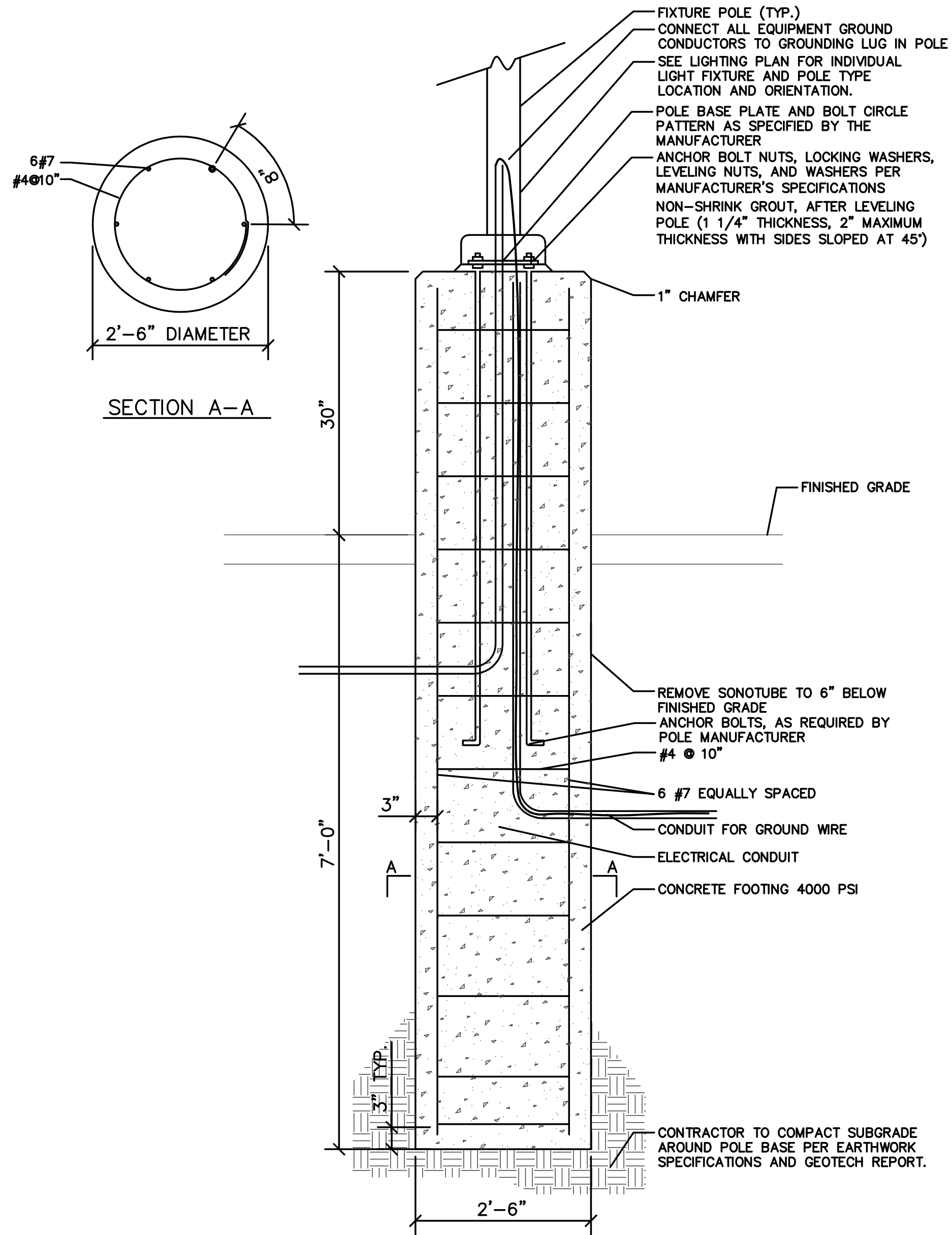
LIGHT POLE DETAIL NTS
