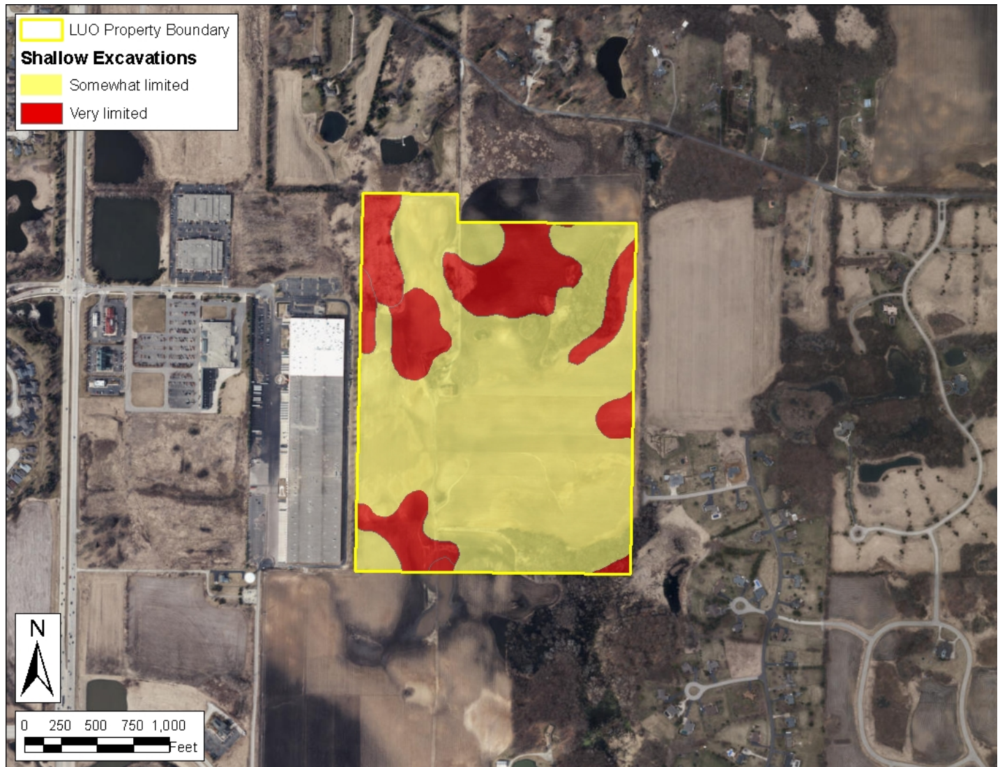
Figure 83: Soil Interpretations for Shallow Excavations
