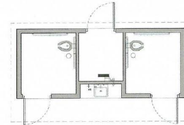
FLOOR PLAN SCALE: NOT TO SCALE
