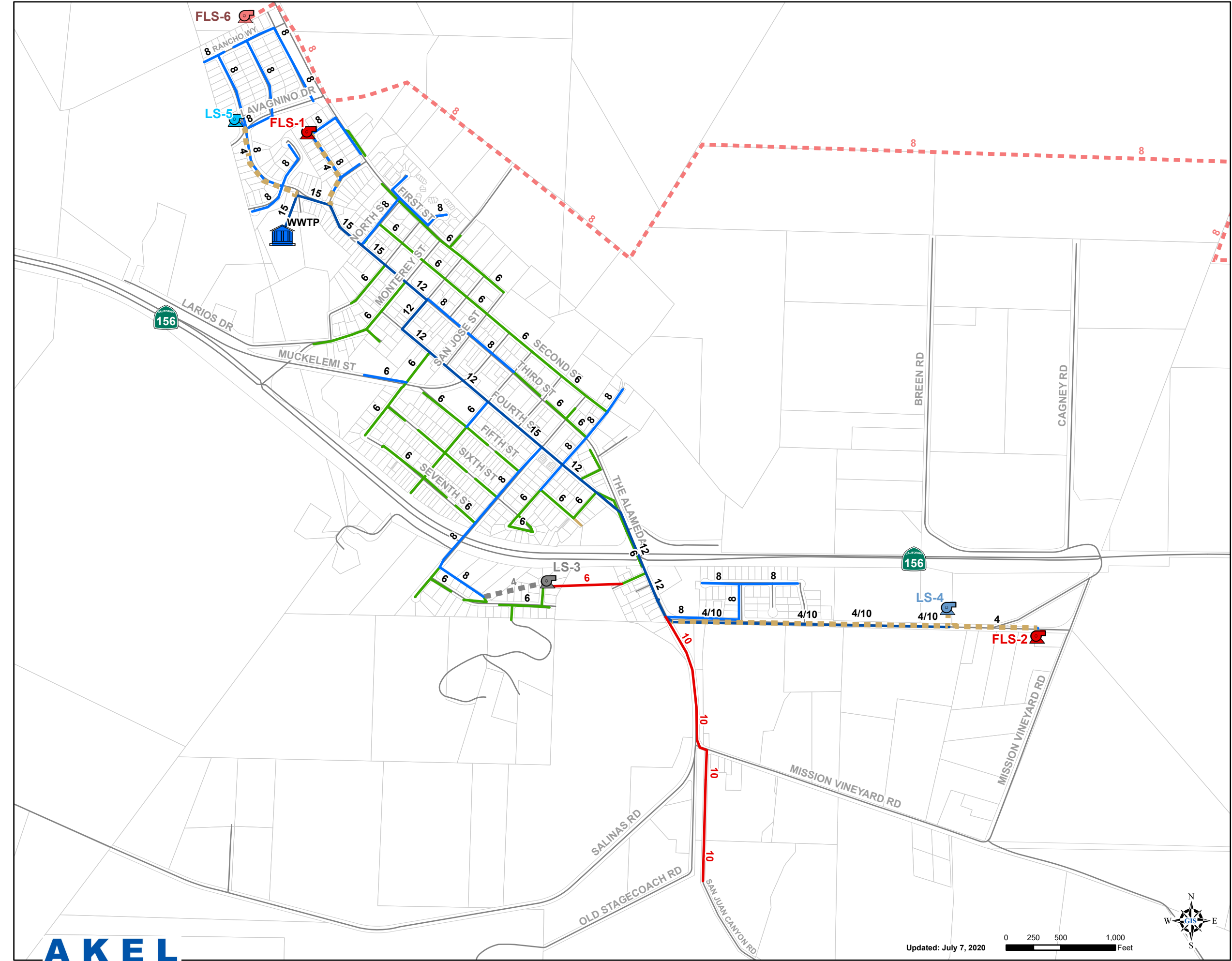
Figure 7.4 Recommended Improvements Wastewater Master Plan City of San Juan Bautista
