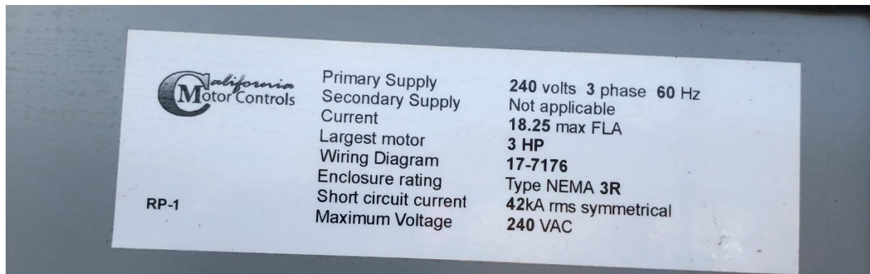
Figure B.3 – Control Panel Information
