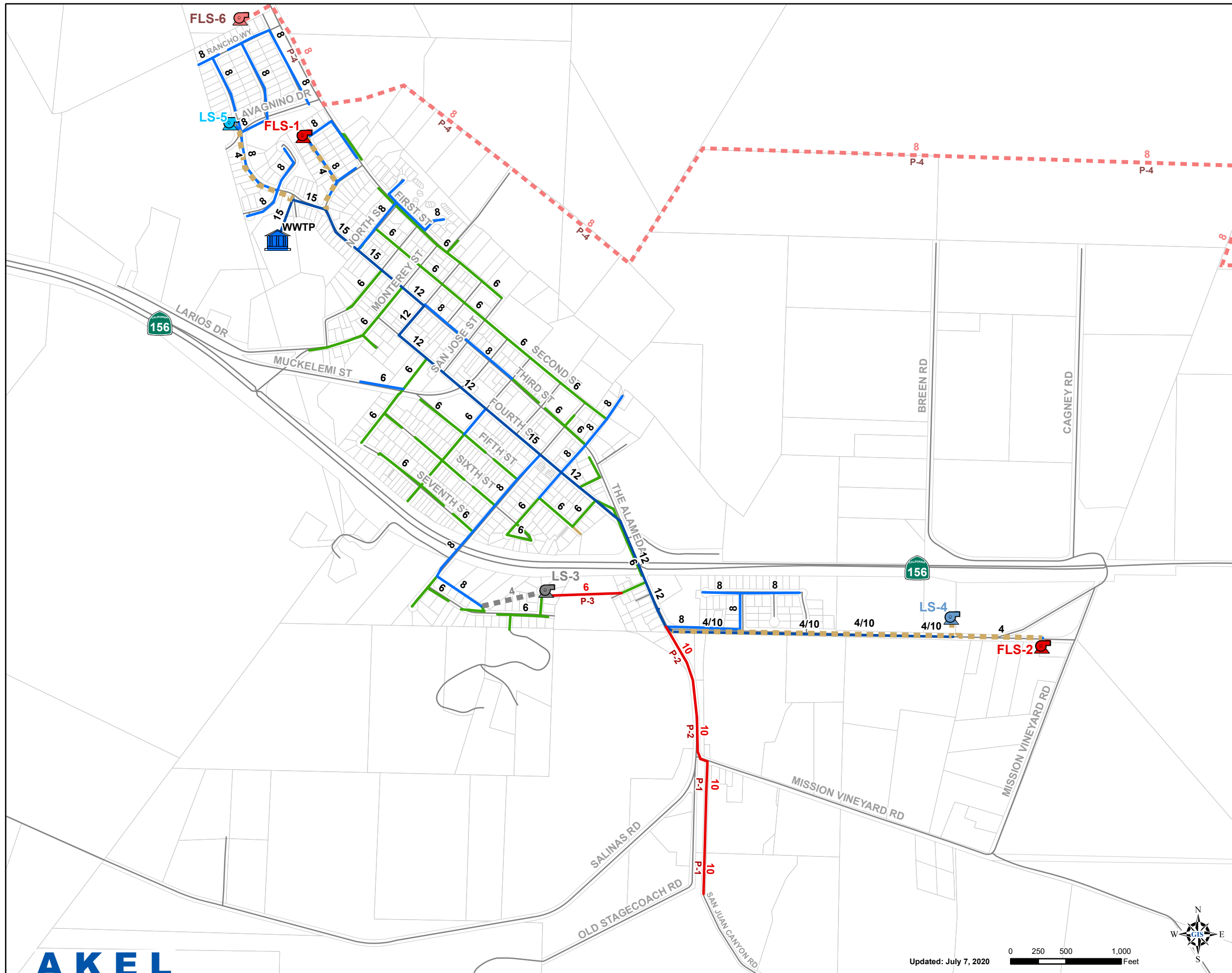
Figure ES.3 Capital Improvement Program Wastewater Master Plan City of San Juan Bautista
