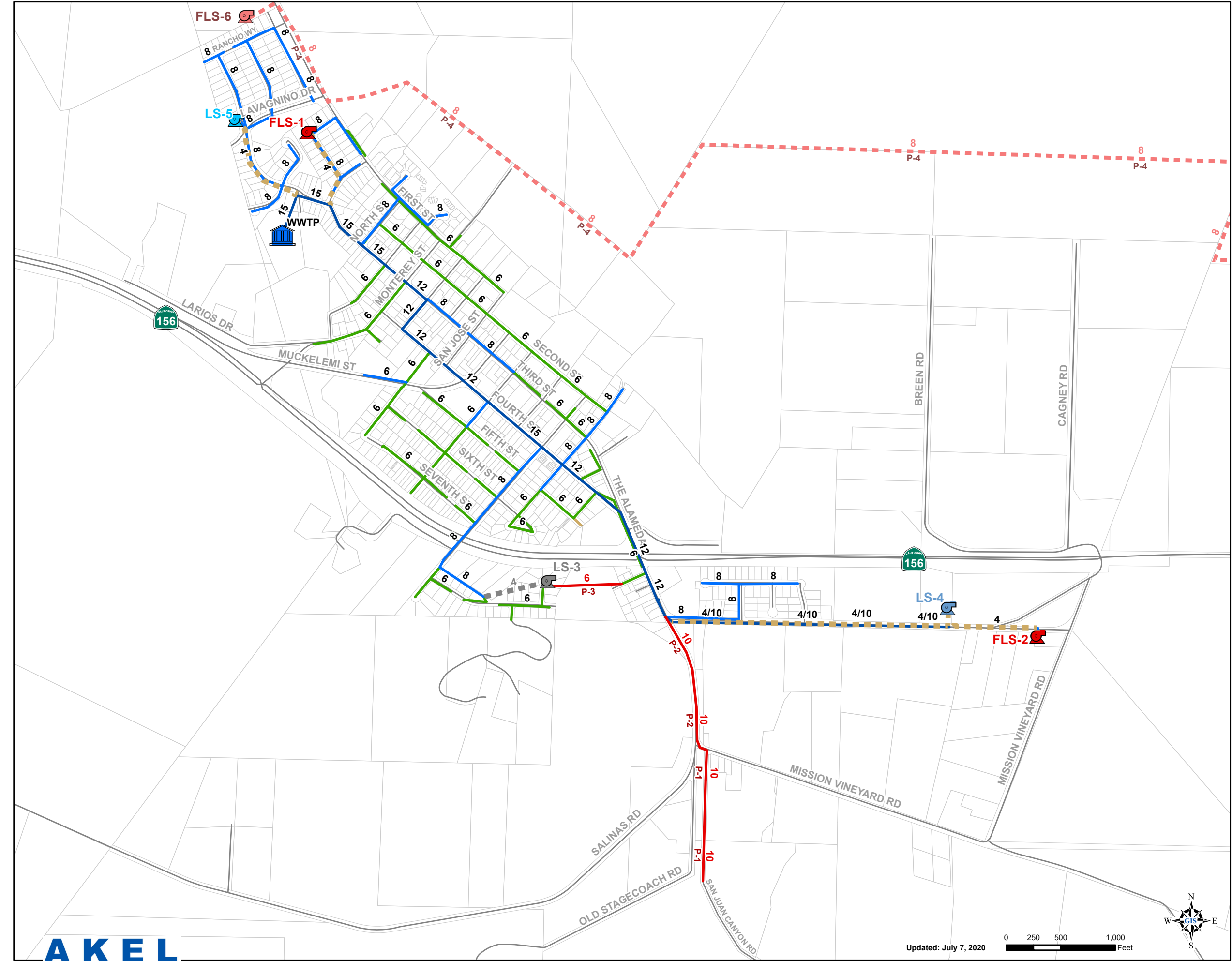
Figure 8.1 Capital Improvement Program Wastewater Master Plan City of San Juan Bautista
