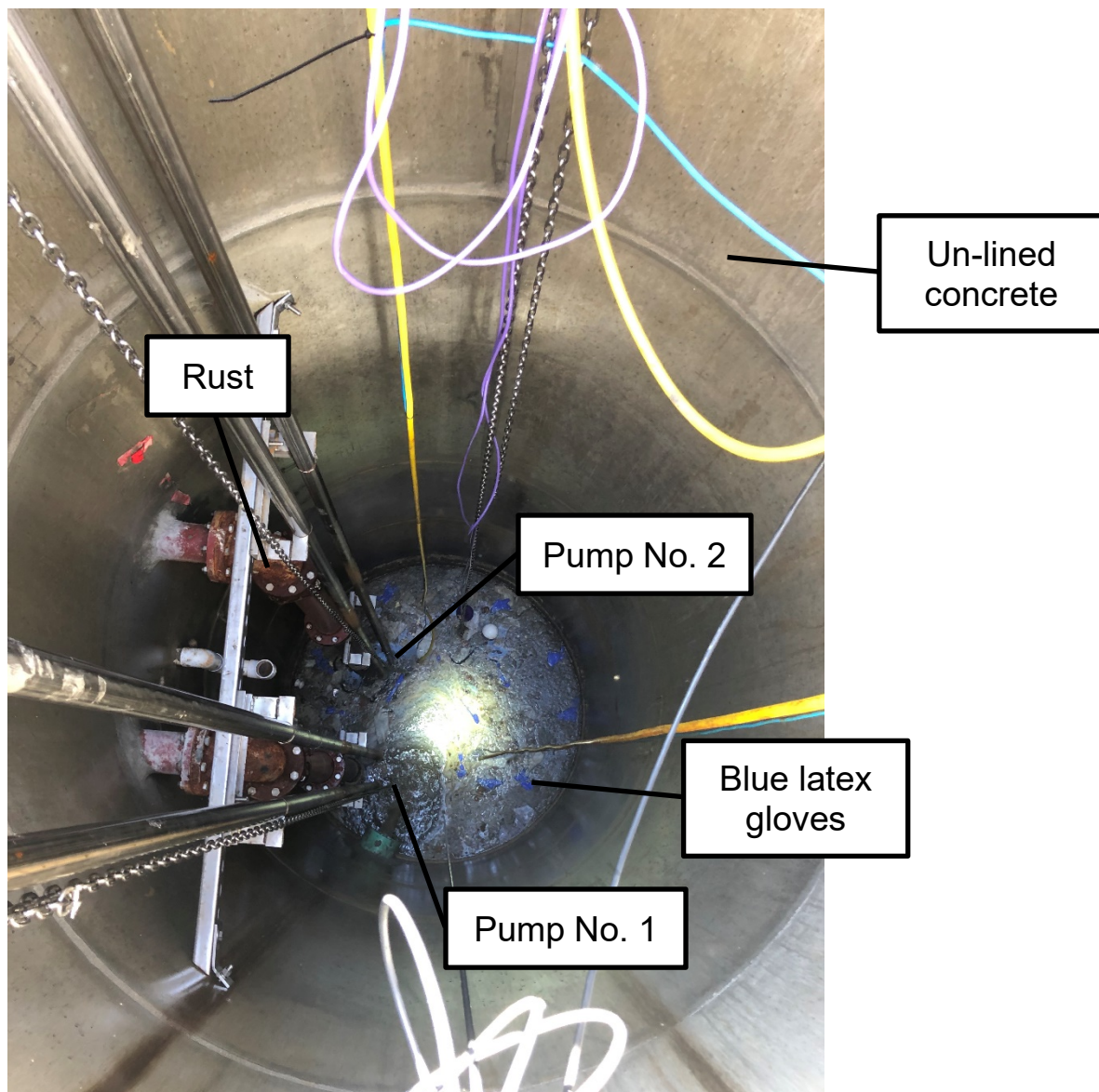
Figure 3 – Inside RVSLS Wet Well
