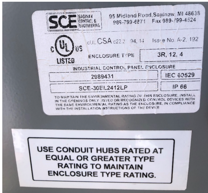
Figure B.4 – Control Panel Enclosure Information
