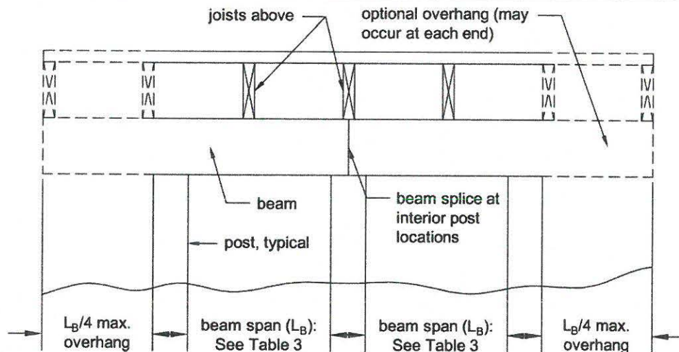
Figure 3. Beam Span.
